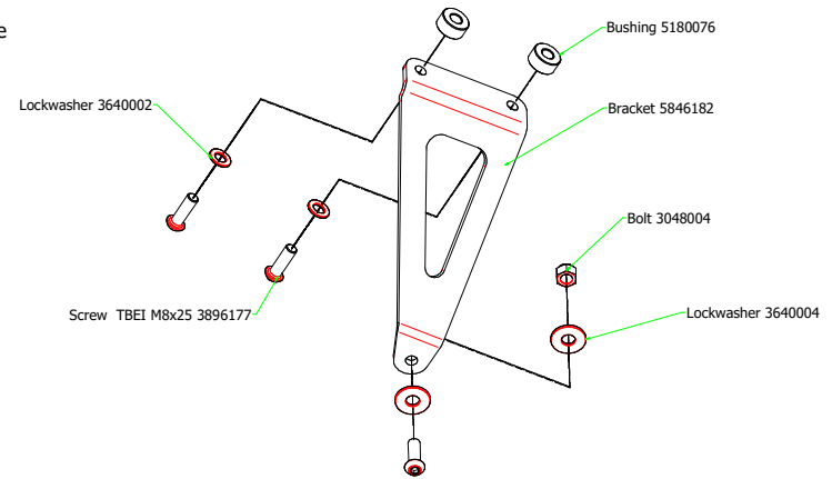
71627MI Racing Link Pipe
