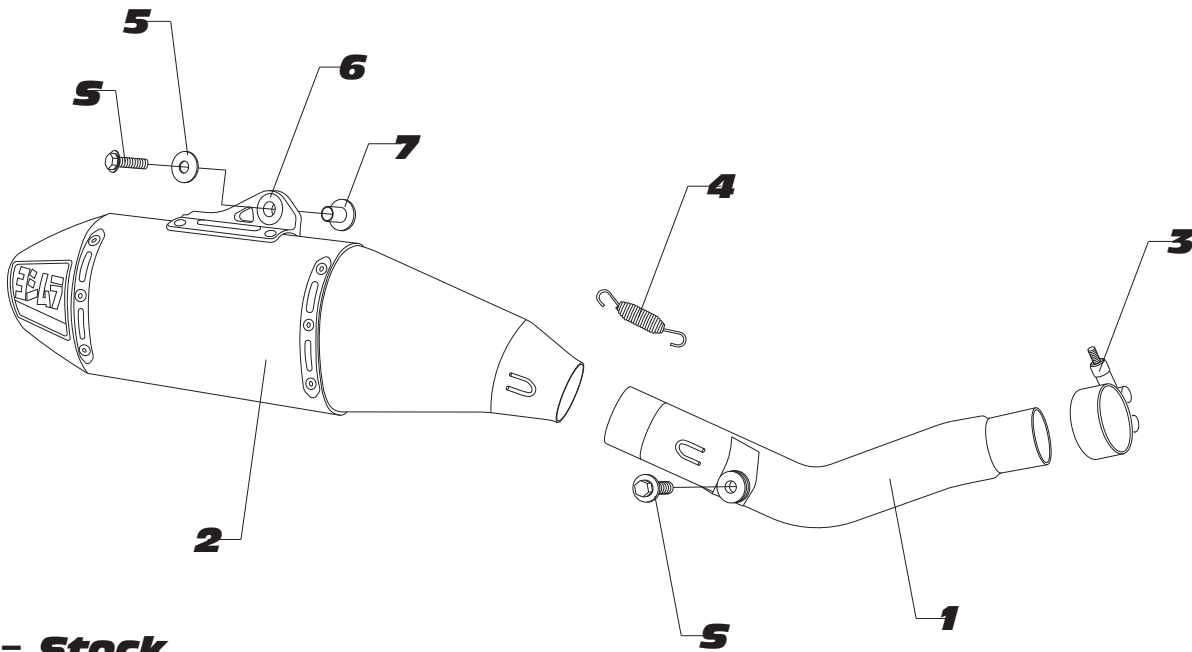
Parts Diagram
