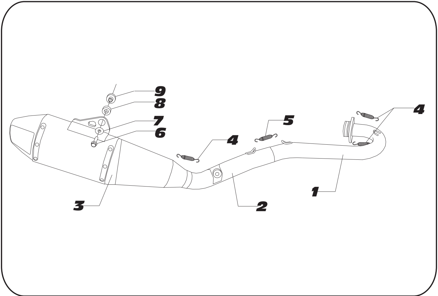
Parts Diagram
